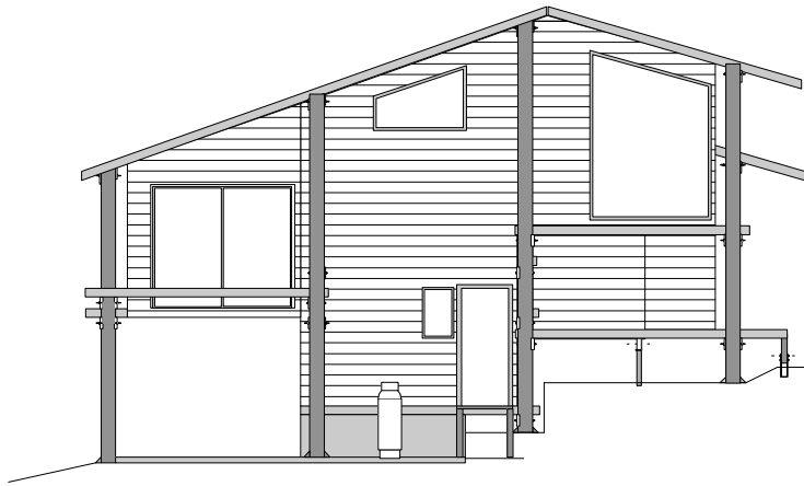
EAST ELEVATION
